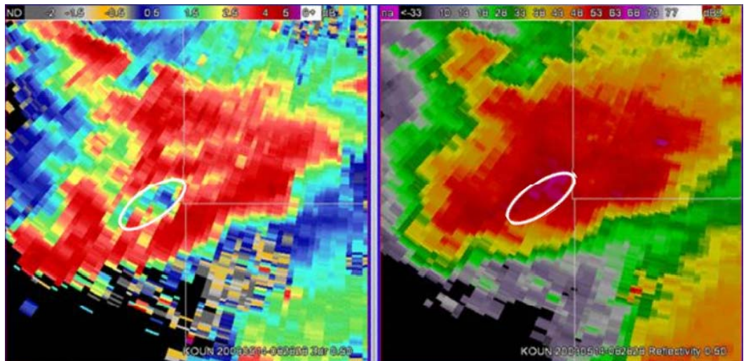
Differential Reflectivity (left), Reflectivity (right). Note white circled area with low differential reflectivity, but high reflectivity.
