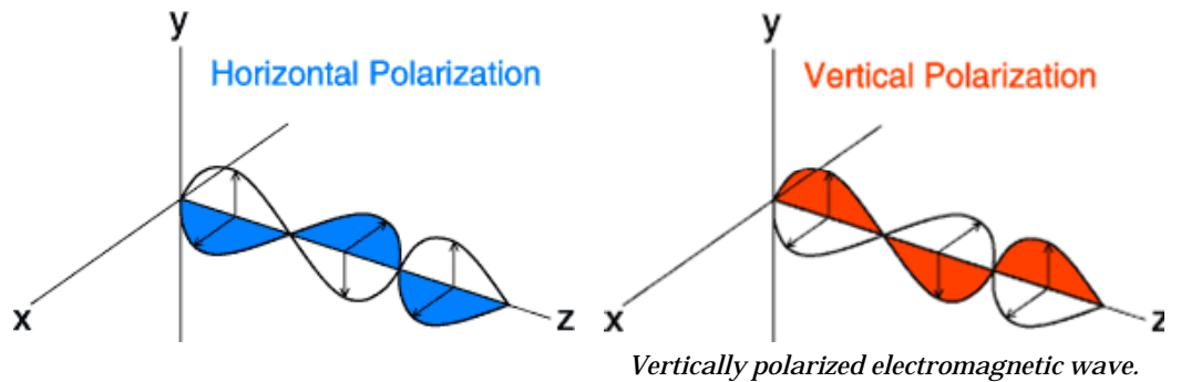
Horizontally polarized electromagnetic wave.
