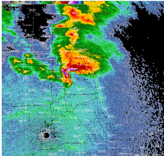
A reflectivity image of storms over northern Cook and southern Lake Counties.
