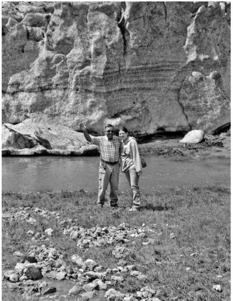
Fig. 6. Hail piled high by a storm near midnight, August 13, 2004, then cut through by floodwater, south of Clayton, New Mexico. Note layering of sediment in the ice "cliff" on the opposite bank.
