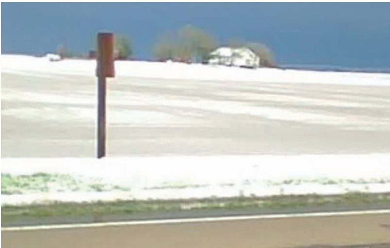
Fig. 5. Deep hail in farm country of the Nebraska Panhandle, late afternoon, June 10, 2009.
